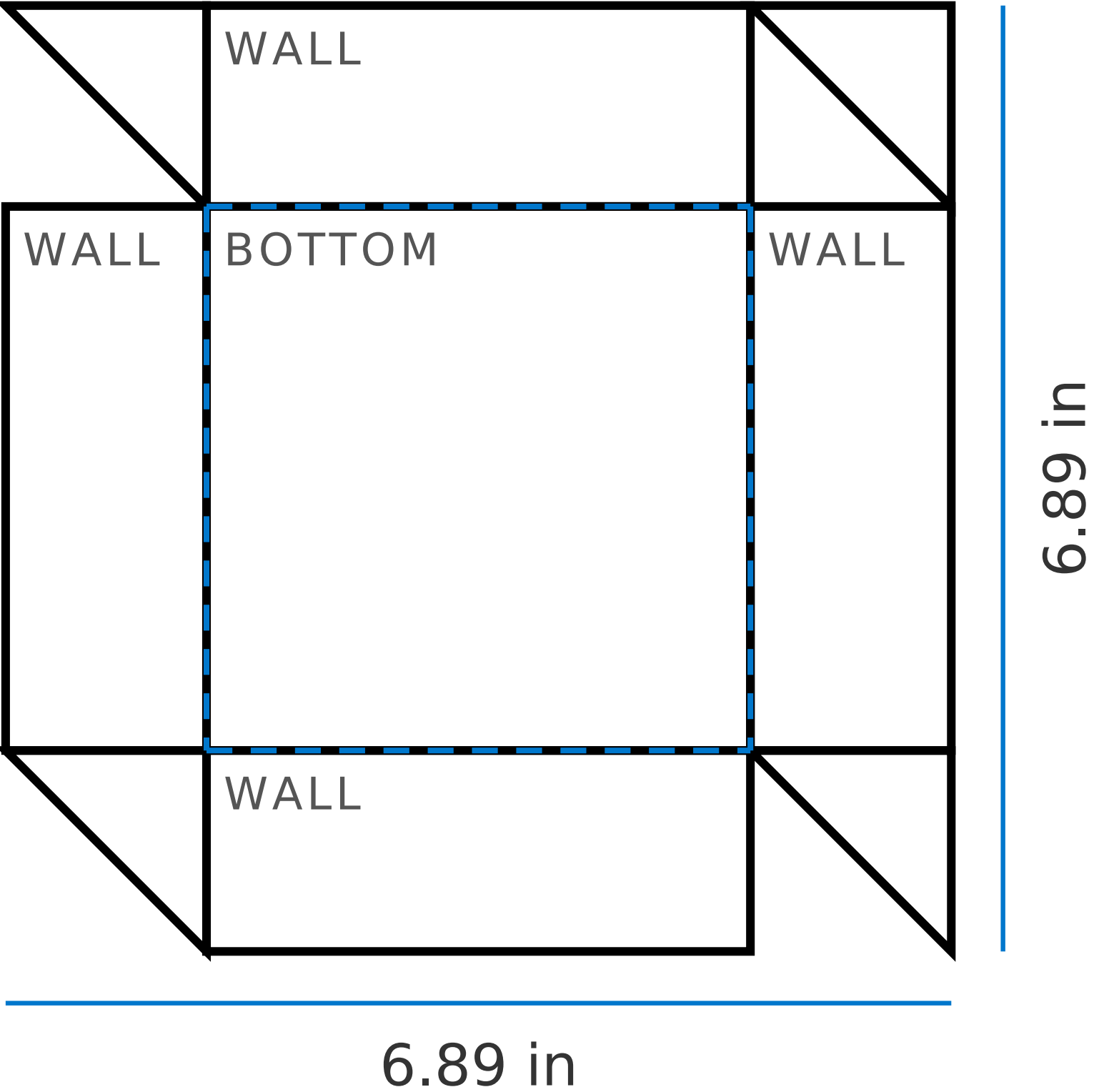
TRAY BLANK, GLUED CORNERS
